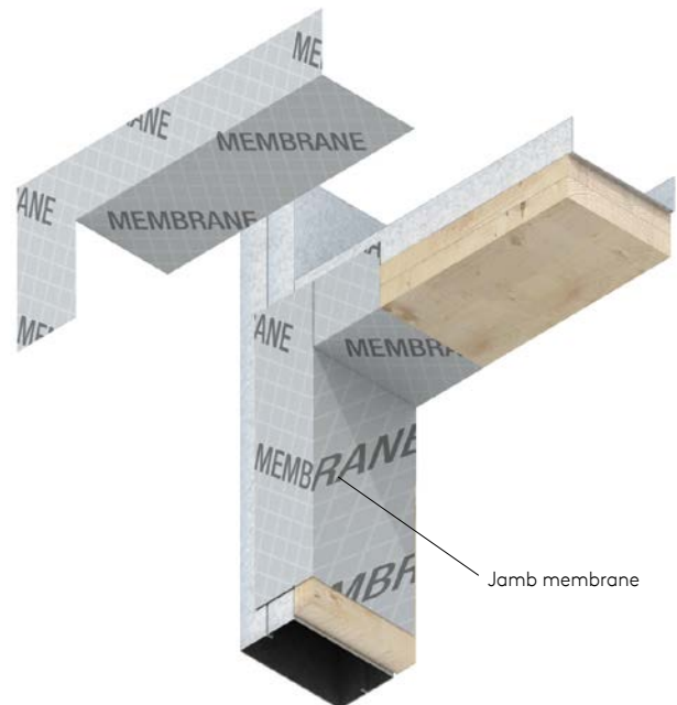
Membrane Corner Patch Self Adhering Membrane
