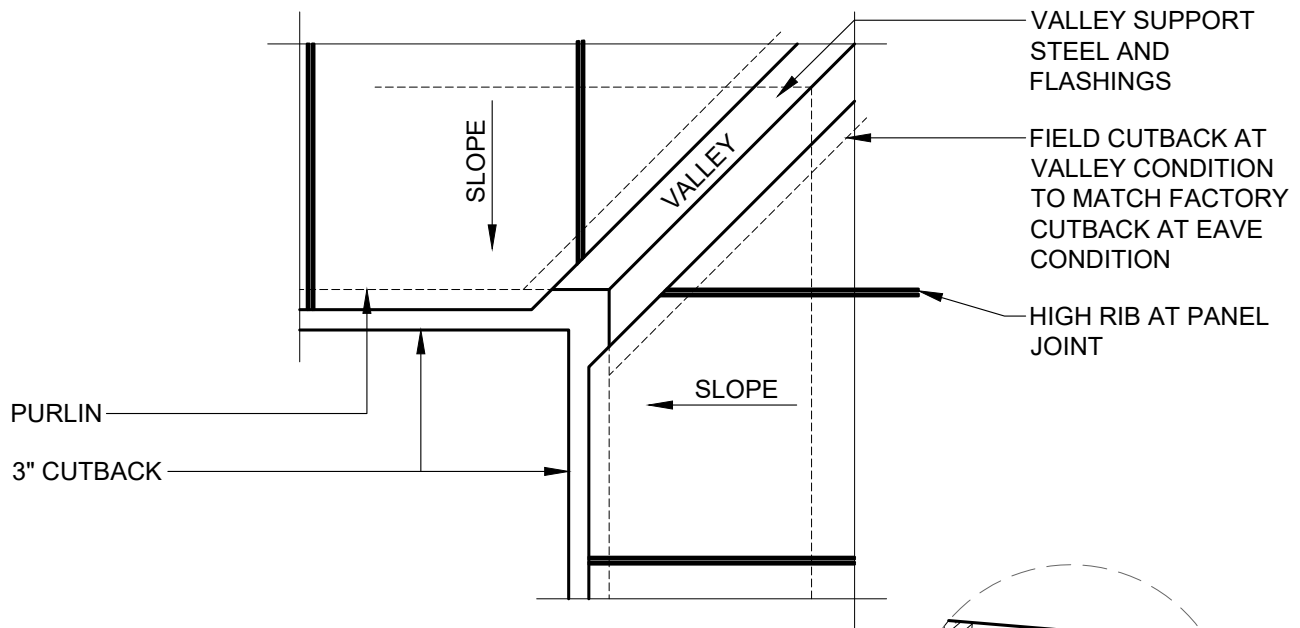
ROOF VALLEY PLAN
