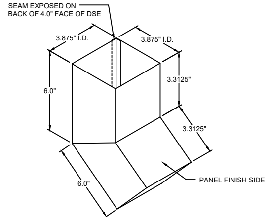
DOWNSPOUT ELBOW - OUTSIDE SEAM XX GA. COLOR (PAINT FINISH) EMBOSMENT BLANK WIDTH: 17.00" X 1'-0" LENGTH 5 BENDS - 0 HEMS
