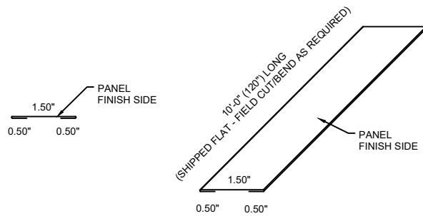
DOWNSPOUT STRAP - FLAT XX GA. COLOR (PAINT FINISH) EMBOSMENT BLANK WIDTH: 2.50" X 10'-0" LENGTH 0 BENDS - 2 HEMS
