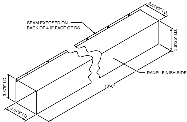
DOWNSPOUT TRIM XX GA. COLOR (PAINT FINISH) EMBOSMENT BLANK WIDTH: 16.75" X 10'-0" LENGTH 5 BENDS - 0 HEMS
