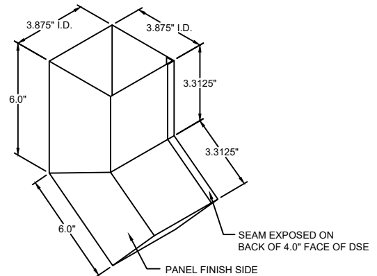
DOWNSPOUT ELBOW - INSIDE SEAM XX GA. COLOR (PAINT FINISH) EMBOSMENT BLANK WIDTH: 17.00" X 1'-0" LENGTH 5 BENDS - 0 HEMS
