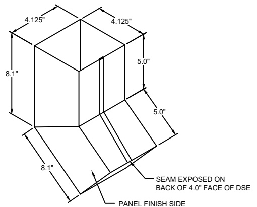
OVERSIZED DOWNSPOUT ELBOW - INSIDE SEAM XX GA. COLOR (PAINT FINISH) EMBOSMENT BLANK WIDTH: 17.00" X 16.20" LENGTH
