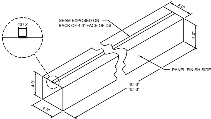
OVERSIZED DOWNSPOUT TRIM XX GA. COLOR (PAINT FINISH) EMBOSMENT BLANK WIDTH: 17.00" X 10'-3" / 15'-3" / 20' MAX. LENGTH
