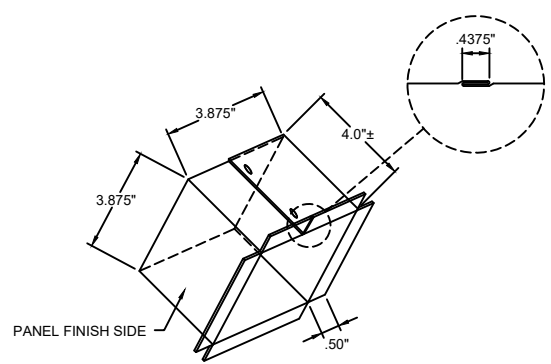
OVERSIZED DOWNSPOUT ADAPTER XX GA. COLOR (PAINT FINISH) EMBOSMENT BLANK WIDTH: 17.00" X 4.5" LENGTH
