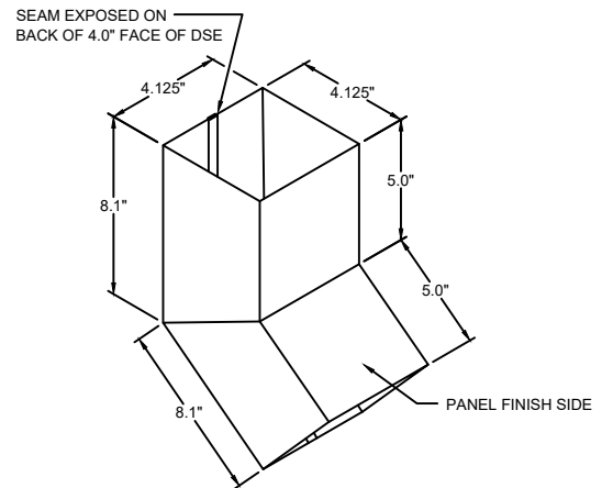
OVERSIZED DOWNSPOUT ELBOW - OUTSIDE SEAM XX GA. COLOR (PAINT FINISH) EMBOSMENT BLANK WIDTH: 17.00" X 16.20" LENGTH
