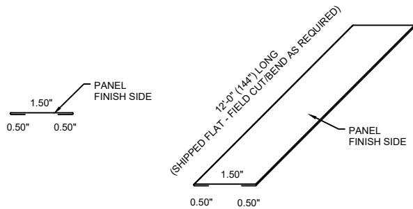
OVERSIZED DOWNSPOUT STRAP - BENT XX GA. COLOR (PAINT FINISH) EMBOSMENT BLANK WIDTH: 2.50" X 12'-0" LENGTH
