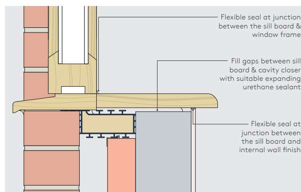
Figure 21: Oversailing window board
