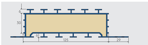
Figure 24: Kingspan Thermabate® 125
