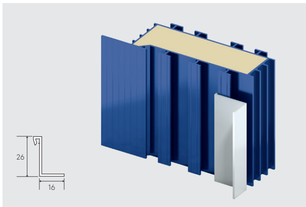
Figure 27: Reveal Clip - White
