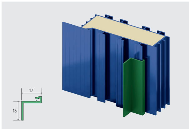
Figure 26: Standard Flange Clip - Green
