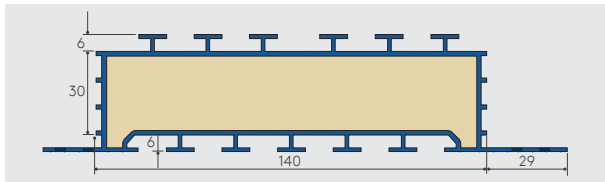
Figure 25: Kingspan Thermabate® 140
