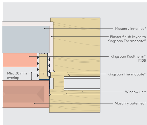
Figure 4: Flush reveal
