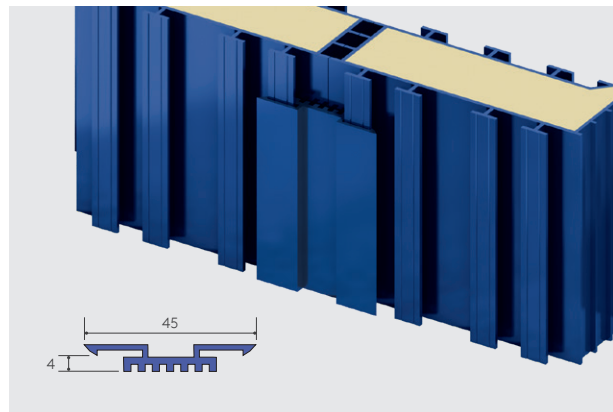
Figure 29: Joining Clip - Blue
