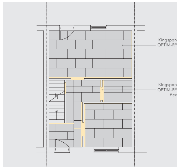
Figure 2: A typical terraced property with a solid concrete ground based floor
