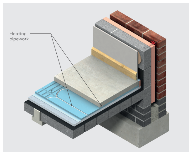
Figure 9: Intermittent heating applications - installed onto beam and block floor underneath screed
